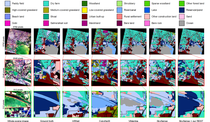
Fig. 4. Visualization of segmentation results on WHU-OHS dataset. Even on the challenging hyperspectral imagery datasets, REST demonstrates better segmentation results than the competing methods. All models use the UPerNet as the decoder. Best viewed in color.
